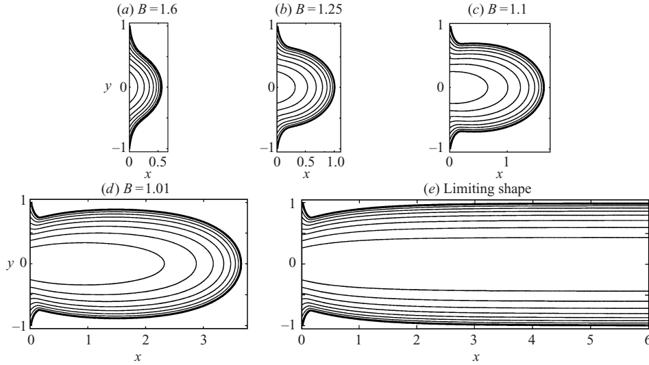
FIGURE 14. Contours of constant height (spaced by 0.1) for stationary rivulets emerged from a Gaussian orifice with half-width y_* = 0.8 . Shown are four values of B , and the limiting shape as B \rightarrow 1 (with S = 1 ).
