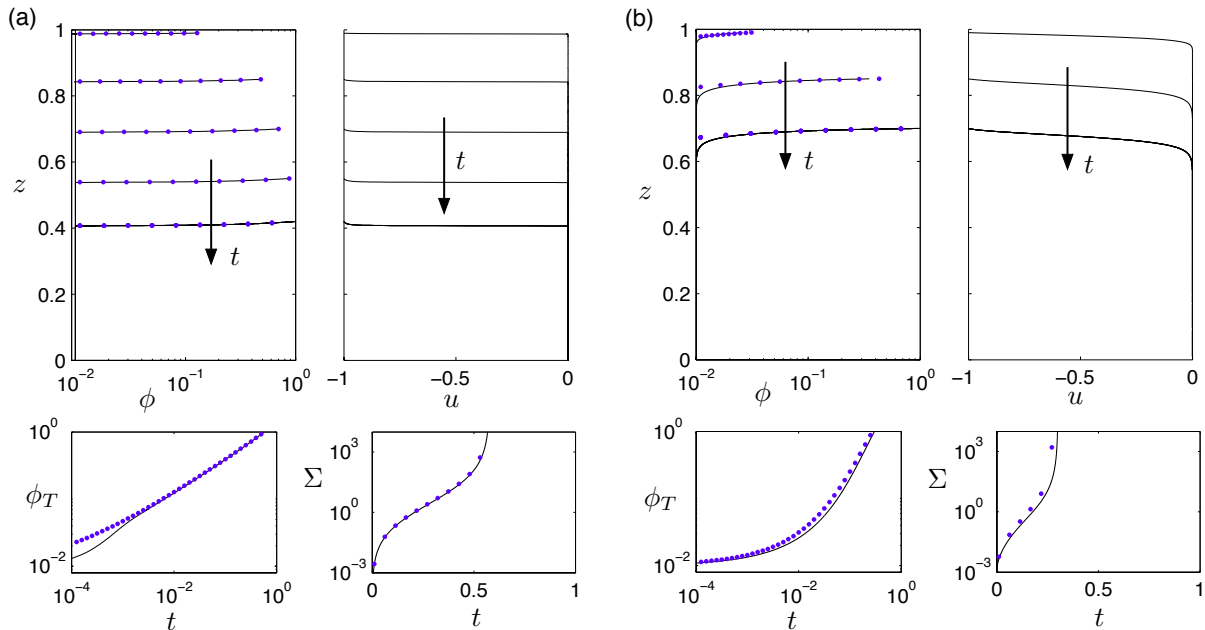
FIG. 4. Solutions for fast compaction exhibiting ‘early-time blow up’, with \phi_0 = 0.01 and \varepsilon = 0 . (a) n = 3 and \gamma = 5 \times 10^{-3} ; (b) n = 1.5 and \gamma = 1 \times 10^{-3} . Snapshots are shown at times t = 0.01, 0.15, 0.3, 0.45, and 0.59 . The panels are as in figure 2, with asymptotic results for \gamma \ll 1 from (22) and (25) shown by blue dots. Note that the load \Sigma diverges as \phi_T \rightarrow 1 .
