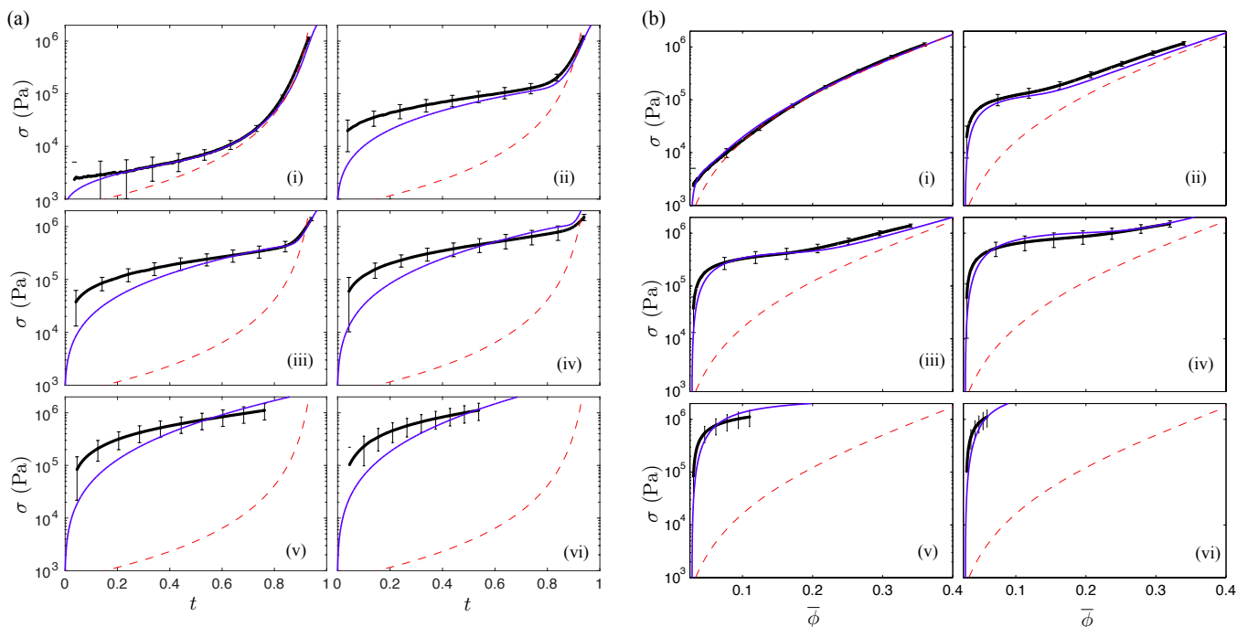
FIG. 7. Average measurements (black solid lines and points) of the load from a suspension of nylon fibres in glycerine, shown (a) as a function of dimensionless time t and (b) as a function of the average solid fraction \bar{\phi}(t) of the suspension, for different speeds U of compression. For each speed, the measurements are averaged over 8 experiments, and the error bars show plus or minus two standard deviations. The different speeds are: (i) U = 0.1 mm/s; (ii) U = 1 mm/s; (iii) U = 2 mm/s; (iv) U = 3 mm/s; (v) U = 4 mm/s; and (vi) U = 5 mm/s. Each panel also shows the theoretical prediction (blue solid) and measured compressive yield stress p_y(\phi) (red dashed; in (a) this is plotted as a function of 1 - \phi_0/\bar{\phi} , which is the dimensionless time for quasi-static compression).
