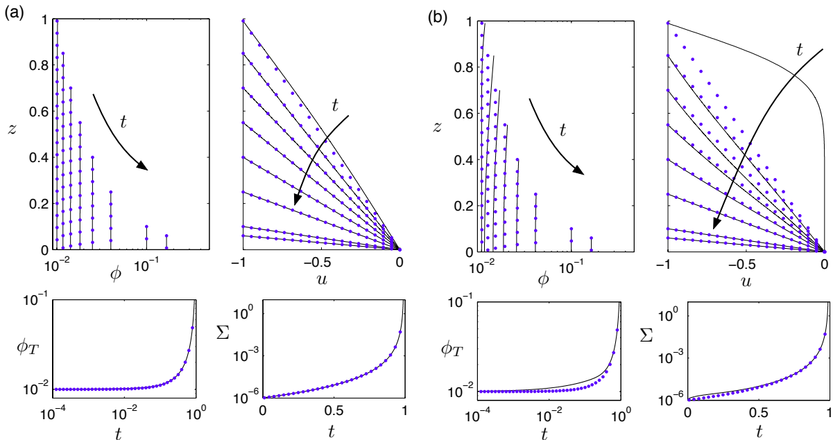
FIG. 2. ‘Slow-compaction’ solutions ( \gamma \gg 1 ) for n = 3 and \phi_0 = 0.01 . (a) \gamma = 10^3 , and (b) \gamma = 50 , together with the leading-order asymptotic predictions for large \gamma (blue dots). Snapshots are shown at times t = 0.01, 0.15, 0.3, 0.45, 0.6, 0.75, 0.9 , and 0.95 . The different panels show the solid fraction \phi (top left), the solid speed u (top right), the solid fraction \phi_T(t) \equiv \phi(z = h) at the piston (bottom left), and the force \Sigma(t) = \Pi_y(\phi_T) at the piston (bottom right).
