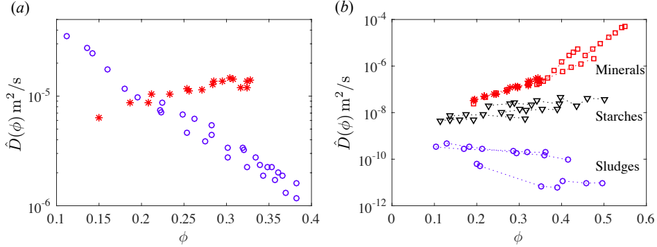
FIG. 6. The dimensional diffusivity function \hat{D}(\phi) = \phi k(\phi) p'_y(\phi) / \mu . (a) Our measurements calculated using the data in figure 5 for nylon fibres in glycerine (red stars) and NBSK cellulose fibres (blue circles). (b) A compilation of some previous measurements for different materials (mineral suspensions, starches and pulps, and sludges and wastewater, as marked), taken from Stickland and Buscall [27] and de Kretser et al. [6].
