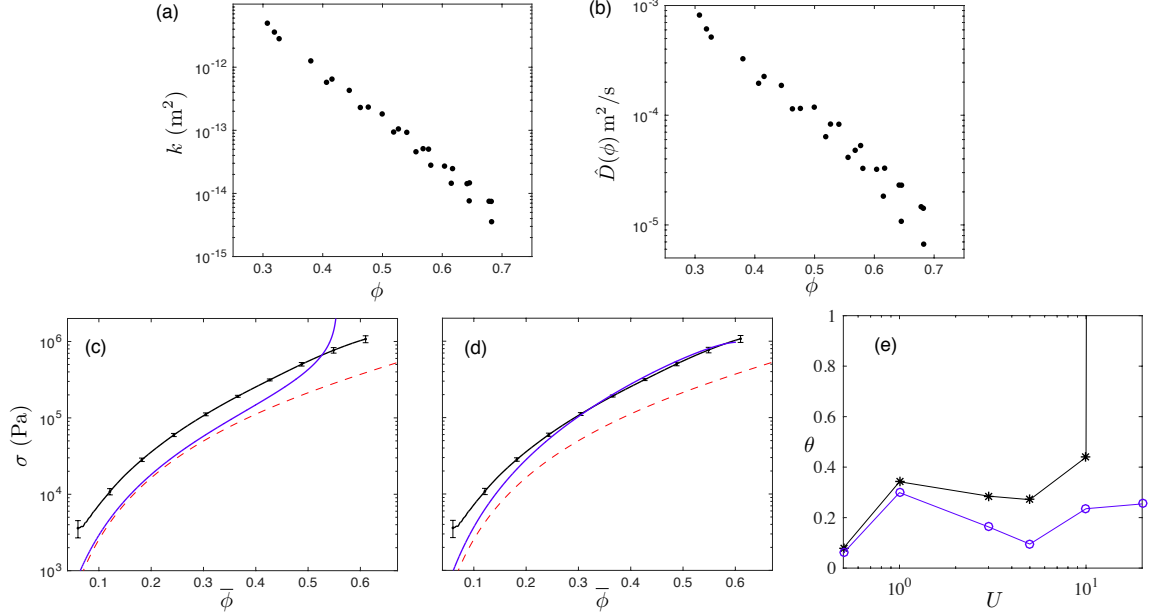
FIG. 15. Results for polyethylene foam in water. (a) The measured permeability k(\phi) . (b) The calculated dimensional diffusivity \hat{D}(\phi) . (c,d) Measurements of the load at speed U = 20 mm/s (black solid), averaged over four experiments, together with the measured compressive yield stress p_y(\phi) (red dashed) and the prediction of the model (blue solid) with: (c) \varepsilon = 0 ; and (d) \varepsilon = 20 . This speed corresponds to a value of \gamma = 1.1 . (e) The goodness-of-fit parameter \theta(U) defined in (33) for the model with \varepsilon = 0 (black stars) and \varepsilon = 20 (blue circles). All simulations with \varepsilon > 0 have \Lambda = \phi^2 .
