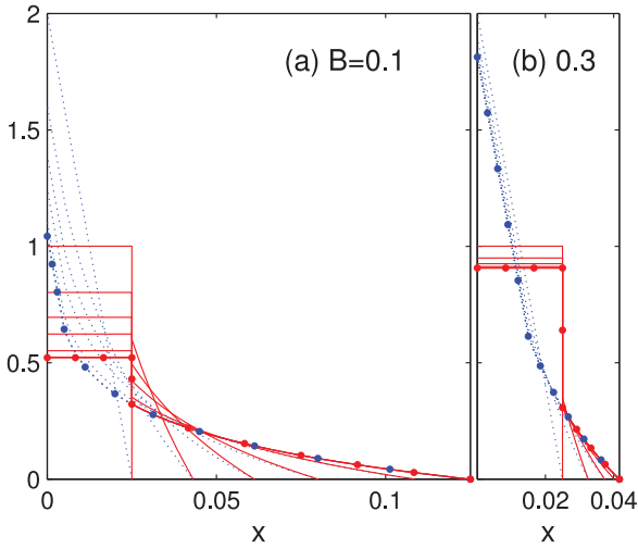
Fig. C.18. Slender asymptotic solutions for (a) B = 0.1 and (b) B = 0.3 , for X_0 = 0.025 , at times t = 0, 4, 9, 16, 36, 100 and 1000 . Collapsing rectangles (triangles) are shown by solid (dotted) lines; the dots indicate the final profiles.
