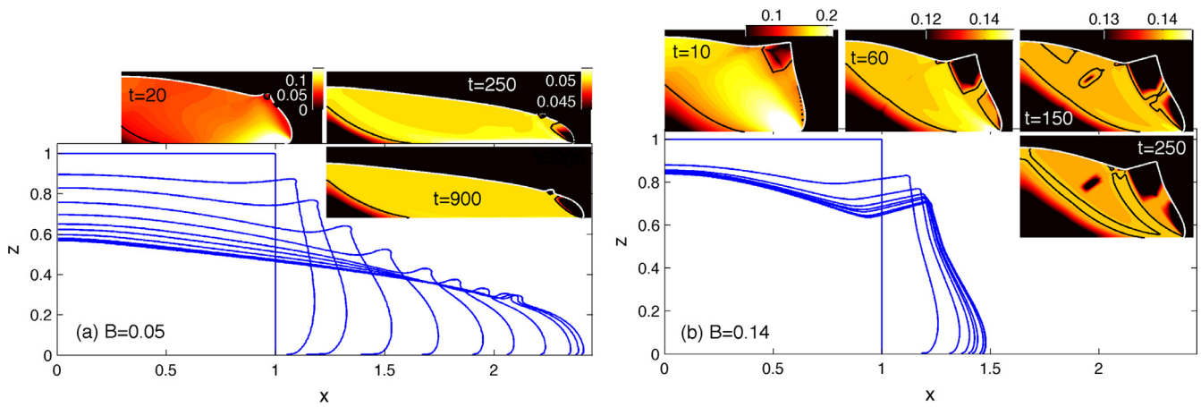
Fig. 5. Snapshots of a collapsing square with (a) B = 0.05 at t = 0, 2.5, 5, 10, 20, 40, 70, 150, 450, 950, 4000 , and (b) B = 0.14 at t = 0, 10, 50, 100, 200, \dots, 1000 . The insets show density plots of the stress invariant \tau at the times indicated, with the yield surfaces drawn as solid lines (and common shading maps for the final two snapshots in each case).
