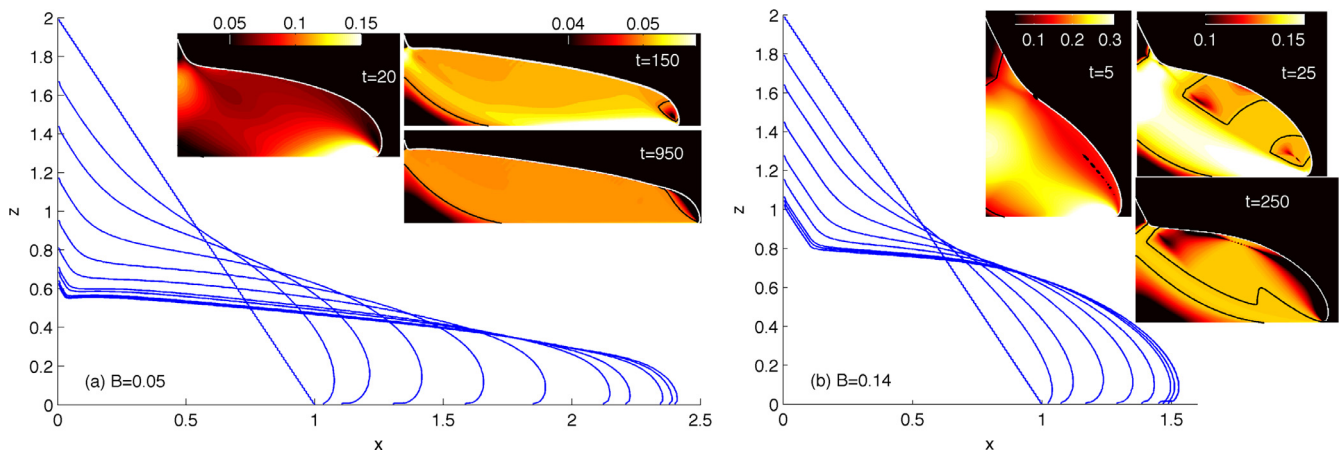
Fig. 6. Snapshots of the evolving interface for a triangular initial condition with X_0 = 1 and (a) B = 0.05 and (b) B = 0.14 , at t = 0, 2.5, 5, 10, 20, 40, 100, 150, 450, 950, 4000 . The insets show density plots of the stress invariant \tau at the times indicated, with the yield surfaces drawn as solid lines (the two later time density plots have a common shading scheme).
