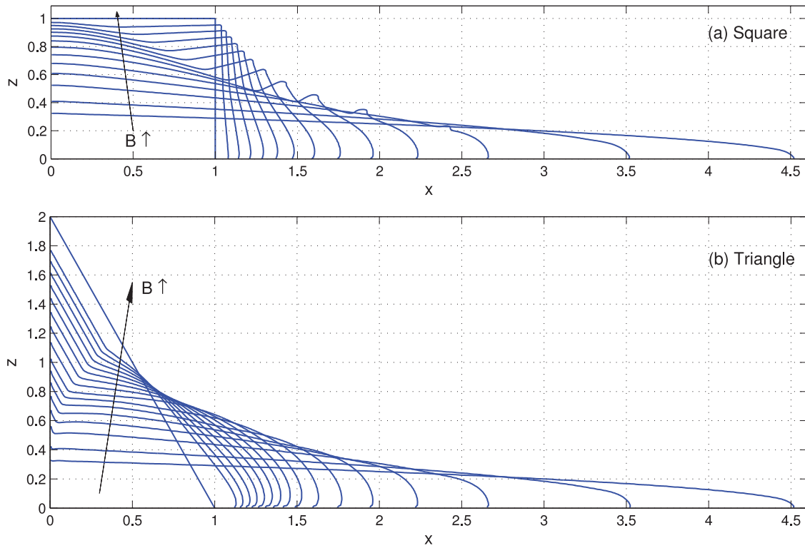
Fig. 14. Profiles of the final deposit, starting from (a) a square block and (b) a triangle, with X_0 = 1 , for B = 0.01, 0.02, 0.04, \dots, 0.22 and 0.24 , together with the initial states.
