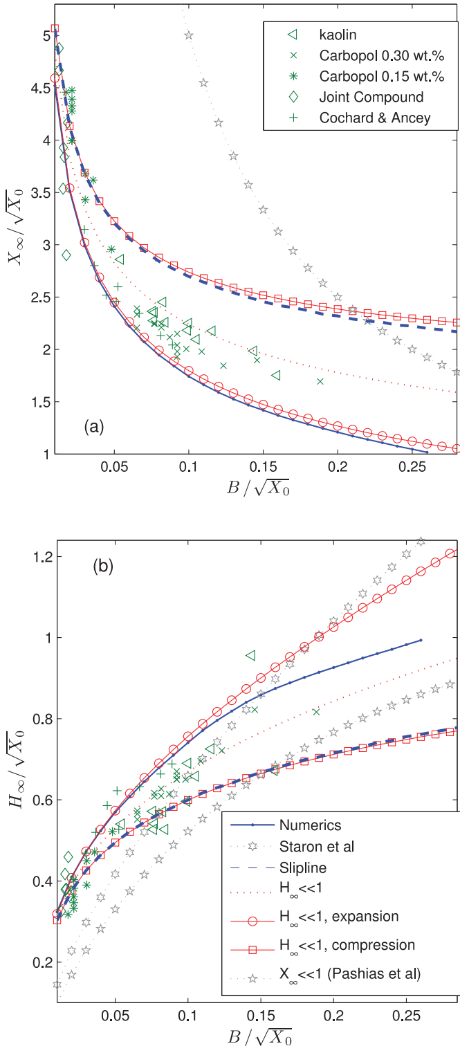
Fig. 16. Scaled final (a) runout X_\infty/\sqrt{X_0} and (b) central depth H_\infty/\sqrt{X_0} as a function of B/\sqrt{X_0} for Bingham slumps from square initial conditions (solid lines with dots). Also plotted using the symbols indicated are experimental data from [17] and [28] for slumps of aqueous solutions of Carbopol, kaolin and “Joint Compound”. The leading order asymptotic prediction (8) is shown by the dotted line; the solid lines with circles or squares plot the predictions in (9) and (13); the dashed lines shows the results of slipline theory [17]. The slender-column asymptotic prediction in (12) with X_0 = 1 is shown by the dotted line and pentagrams. The dotted line and hexagrams show the fit proposed by Staron et al. [6].
