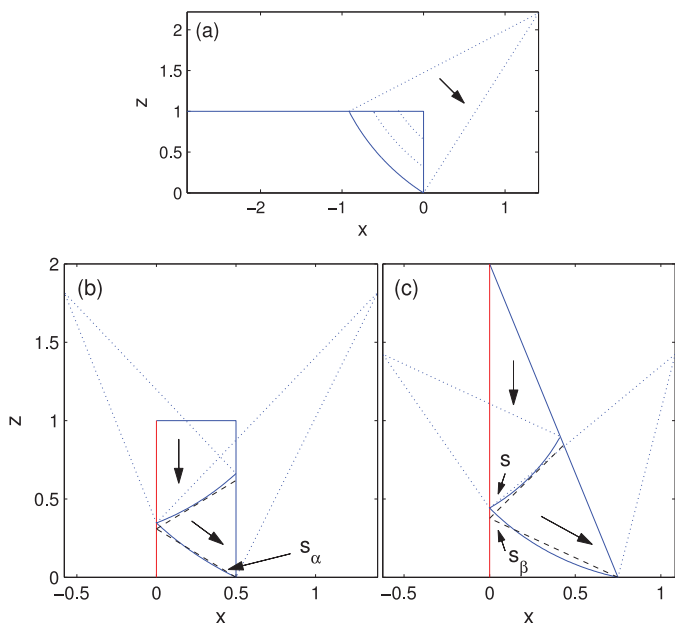
Fig. 11. Trial velocity fields to compute lower bounds on B_c for (a) the vertical embankment with a circular slip curve, and relatively slender (b) rectangular and (c) triangular initial blocks. In (b) and (c), the straight (dashed) and circular (solid) failure surfaces for linear or rotational sliding motion are plotted; these surface can be parametrized by the local slopes at the bottom corner, s_\alpha , and midline, s_\beta and s (for linear sliding s_\alpha = s_\beta ).
