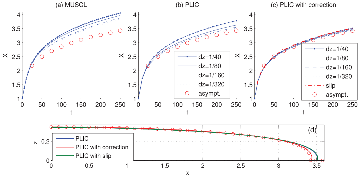
Fig. 3. Flow front X(t) plotted against time for computations with Newtonian fluids using (a) the simple MUSCL scheme, (b) the PLIC improvement, and (c) the PLIC scheme with the lower boundary condition on c(x, z, t) adjusted according to the algorithm outlined in the main text. In each case, runs with different resolution are shown. For (c), the (red) dashed-dotted line labelled slip shows a solution computed with the PLIC scheme, but with no slip imposed on the heavier fluid and free slip imposed on the lighter fluid at z = 0 . The circles show the prediction of the leading-order, shallow-layer asymptotics in Appendix B. In (d), we plot the interface shape at t = 250 for the highest resolution solutions computed with the PLIC scheme with the three different lower boundary conditions.
