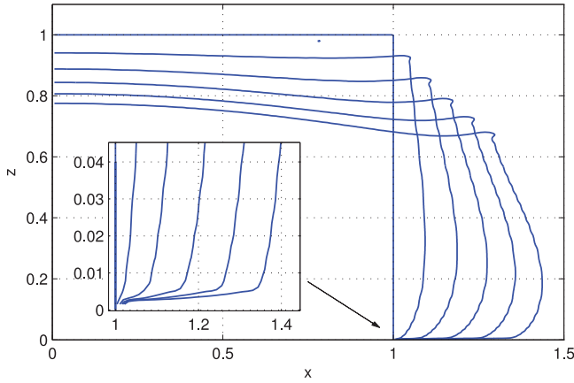
Fig. 2. Snapshots of the evolving interface for a Newtonian heavier fluid at the times t = 1, 2, 3, 4, 5 ; the inset shows a magnification of the finger of over-ridden lighter fluid.
