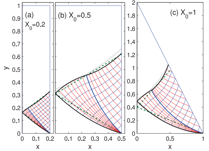
Fig. D.19. Slipline solutions for a rectangle with (a) X_0 = 0.2 and (b) X_0 = 0.5 , and a triangle with X_0 = 1 . The dashed and dotted lines indicate the lower bound and its improvement of D.2.
