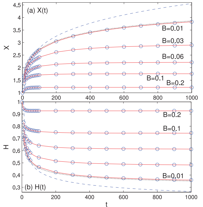
Fig. 4. (a) Front position X(t) and (b) central depth H(t) = h(0, t) for Bingham dambreaks with a square initial block ( X_0 = 1 ) and the values of B indicated. The dashed lines show the Newtonian results. For the viscoplastic cases, the circles show the result using the augmented-Lagrangian scheme and the lines indicate the result with a regularized constitutive law. The dotted lines show the prediction of the leading-order shallow-layer asymptotics for B = 0.01 .
