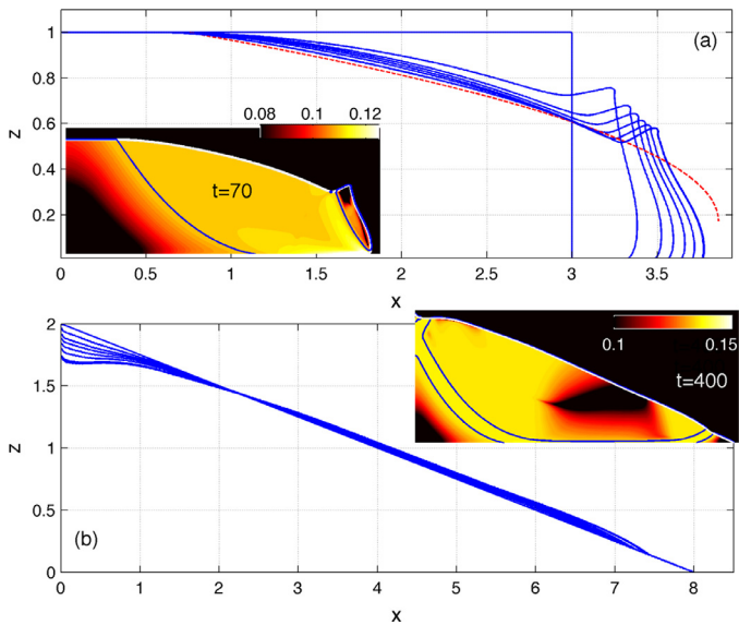
Fig. 7. Snapshots of the evolving interface for an initial (a) rectangular with (X_0, B) = (3, 0.11) , and (b) triangle with (X_0, B) = (8, 0.14) , at the times t = 0, 10, 20, 30, 50, 100, 400, 700, 1000 . The dotted line in (a) shows a modification of the prediction in (9) that incorporates the central plug (and which terminates at finite height). The insets show density plots of the stress invariant \tau at the times indicated, with the yield surfaces drawn as solid lines.
