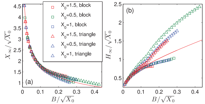
Fig. 17. Scaled final (a) runout X_\infty/\sqrt{X_0} and (b) central depth H_\infty/\sqrt{X_0} as a function of B/\sqrt{X_0} for Bingham slumps from rectangular and triangular initial conditions with X_0 = 0.5, 1 and 1.5 . The solid lines show the predictions of the higher-order asymptotics from (9) for a complete slump.
