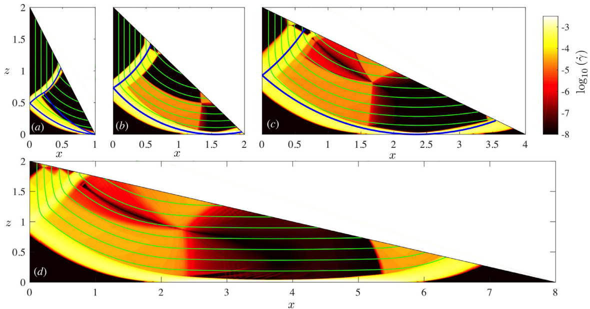
Fig. 13. A series of pictures similar to Fig. 12, but for initial triangles (with solid blue lines showing the yield surfaces of the slipline solution in (a), and the circular arcs of the bound of D.2 for rotational failure in (b) and (c)).
