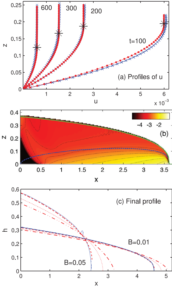
Fig. 9. Comparison of shallow-layer theory with numerical results for a collapsing square block ( X_0 = 1 ) with B = 0.01 : (a) Horizontal velocity profiles at x = 2.5 and the times indicated. (b) Logarithmic strain-rate invariant, A density map of \log_{10} \dot{\gamma} on the (x, z) -plane, at t = 600 . (c) Final shape. In (a) the crosses plot the numerical solution, and the points indicate the asymptotic profile (B.2); the star locates the bottom of the pseudo-plug. In (b), the solid (green) and dashed (blue) lines show the surface and fake yield surface ( z = Y = h + B/h_x ) predicted by asymptotics. In (c), the final profile for B = 0.05 is included. The solid lines show computed final states, the dotted lines denote the leading-order result (8) and the dashed line shows the higher-order prediction (9). The dashed-dotted line is the asymptotic prediction (13) from [17]. (For interpretation of the references to colour in this figure legend, the reader is referred to the web version of this article.)
