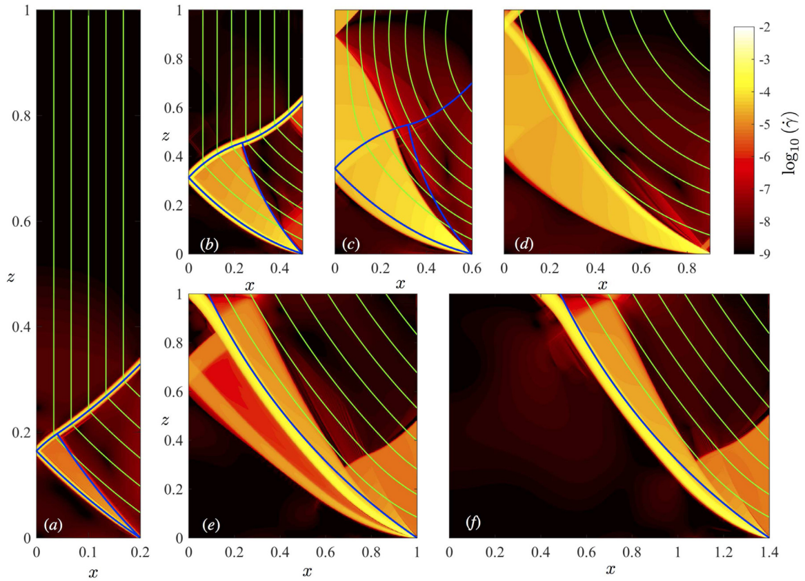
Fig. 12. Strain-rate invariant plotted logarithmically as a density on the (x, z) -plane for solutions with B = 0.99B_c and t = Re = 0 (A.2), at the values of X_0 indicated by the x -axis. Also shown are a selection of streamlines. In (a)–(c), the darker (blue) lines indicate the border of the plastic region and expansion fan of the corresponding slipline solutions (Appendix D). In (e) and (f), the darker (blue) lines indicate the circular failure surface of the lower bound solution. (For interpretation of the references to colour in this figure legend, the reader is referred to the web version of this article.)
