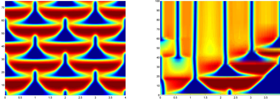
Figure 4: Sensitivity to initial conditions. The left and right figure differ only in the initial conditions. On the left, symmetric initial conditions result in an intricate a time-periodic solution. On the right, the initial condition is the same as on the left, except for a shift of 0.1 units to the right. dynamics eventually settle to a 5-spike stable pattern. Parameter values for both figures are \rho = 7, d_2 = 0.0005, (a_1, b_1, c_1) = (5, 1, 1); (a_2, b_2, c_2) = (1, 1, 2) .
