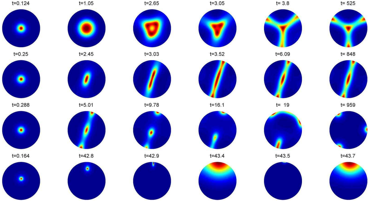
Figure 5: Various dynamics observed in two dimensional disk. Parameter values are as given by (94) except for \rho as specified below. Row 1: \rho = 2 . Spot splits into three spots. Row 2: \rho = 4 . Initially, spot splits into two, final steady state consists of two boundary and one center spot. Row 3: \rho = 6 . Row 4: \rho = 500 . The interior spike is unstable and slowly drifts to the boundary. Once it reaches the boundary, it starts to oscillate indefinitely.
