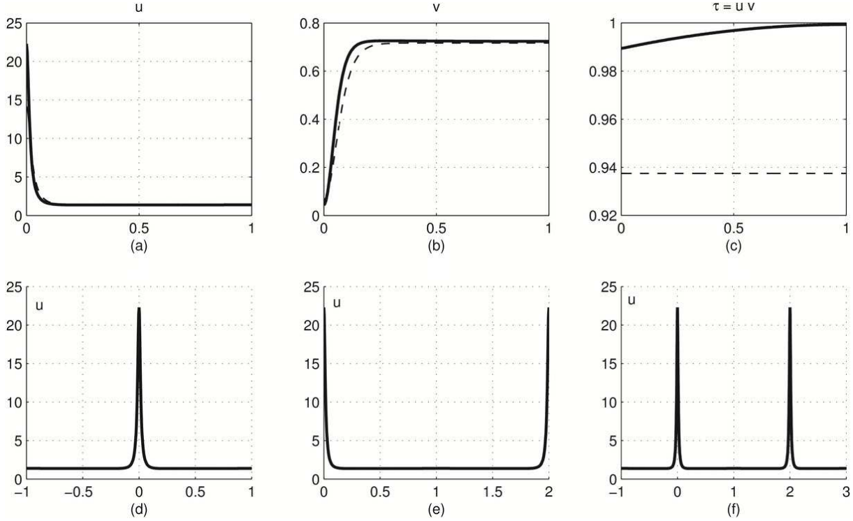
Figure 1: Steady states configurations considered in this paper. (a,b,c): Half-spike on [0, L] . Both u and v have boundary layers at zero, whereas \tau = uv is nearly constant. Note that v(0) is small and u(0) is large. Solid line shows the full numerical computation; asymptotic approximations derived in Proposition 2.1 are shown using dashed line. Parameter values are d_2 = 4 \times 10^{-3} , \rho = 200 , (a_1, b_1, c_1) = (5, 1, 1) , (a_2, b_2, c_2) = (5, 1, 5) and L = 1 . (d) A single interior spike; (e) A double-boundary spike configuration; (f) a two-spike configuration (i.e. L = 1, K = 2 ).
