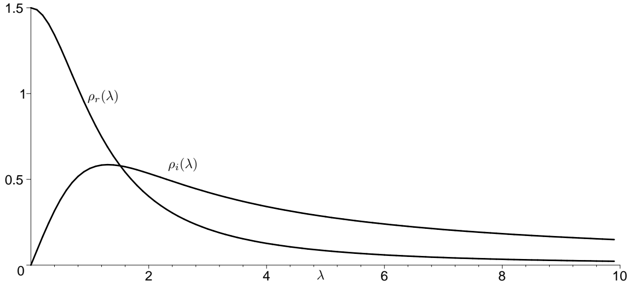
Figure 3: Graphs of \rho_r(\lambda) and \rho_i(\lambda)
