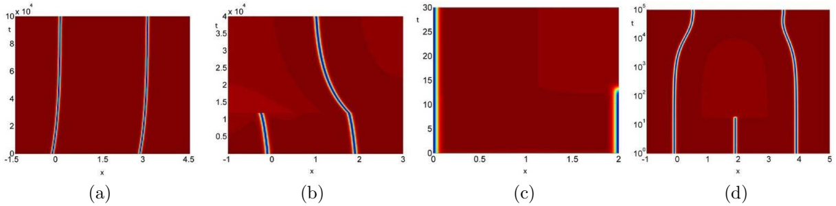
Figure 2: Various instabilities of Principal Result 1.1. (a) Two stable spikes. Parameter values in (2) are d_2 = 10^{-3} , \rho = 200 , (a_1, b_1, c_1) = (5, 1, 1) , (a_2, b_2, c_2) = (5, 1, 5) and L = 1.5 , K = 2 , with b - a = 2KL . (b) Slow instability: two spikes persist as a transient state until t \sim 1.2 \times 10^4 . Parameter values are the same as (a) except that L = 1 . (c) Fast instability of two boundary spikes: Parameter values are the same as (b), except that b - a = 2 . (d) Fast instability of three spikes (note log time scale): the middle spike disappears at t \sim 20 . The remaining two spikes slowly drift towards a symmetric equilibrium. Parameter values are the same as (b) except K = 3 .
